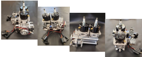
GZR 54.4cc 2022 Billit PRO-MOD IN-LINE racing engine
